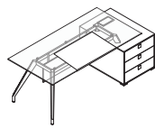
ARDGS R/L ARSU L180 W90 H75 L200 W90 H75 L220 W90 H75 L63 W90 H60
