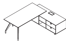
ARDS R/L ARSU R/L L180 W90 H75 L200 W90 H75 L220 W90 H75 L168 W65 H60
