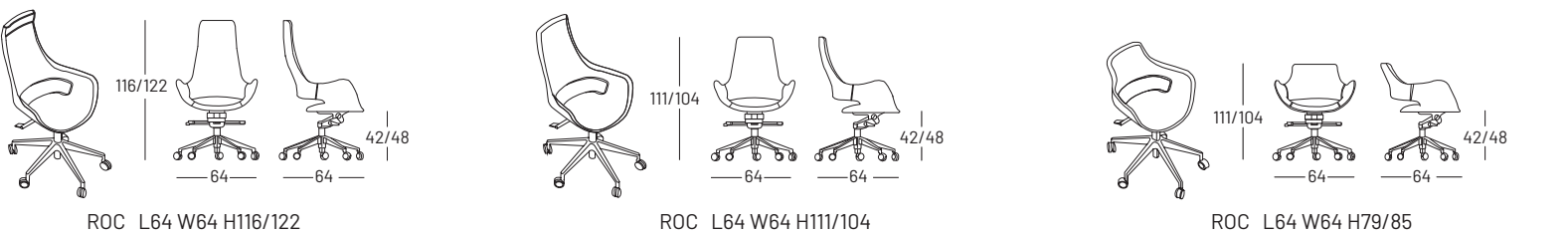
Adjustable height waiting chair - Spider leg visitor chair - Cantilever visitor chair - Four leg visitor chair
