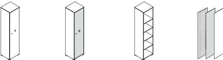
Internal Cabinets L47 W43 H197 - Back
