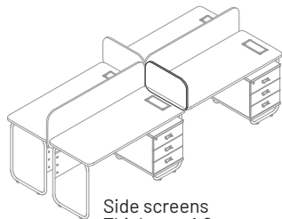
Side screens Thickness 1.8 RTSS L60 H39 L80 H39
