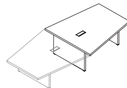
End part with side leg and central leg L160 W120/160 H75 CLTML L200 W120/160 H75
