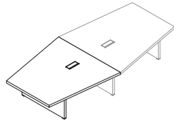
End part with side leg L160 W120/160 H75 CLTME L200 W120/160 H75
