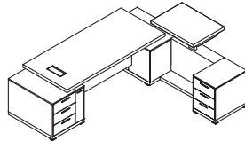
CLDT CLSU R/L L65 W90 H65 L180 W90 H75 CLSUA R/L L228 W65 H65 L200 W90 H75 L220 W90 H75
