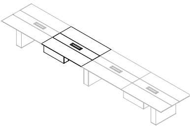
Middle top 2 with wood box VIMMT2 L160 W120 H75
