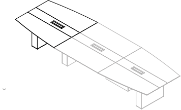
End top with marble boxes VIMETT L160 W120/160 H75 L200 W120/160 H75 L180 W120/160 H75 L220 W120/160 H75
