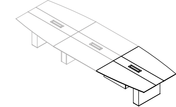
Start top with marble & wood boxes VIMSTT L160 W120/160 H75 L200 W120/160 H75 L180 W120/160 H75 L220 W120/160 H75
