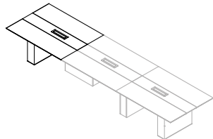
End top with marble boxes VIMET L160 W120 H75 L200 W120 H75 L180 W120 H75 L220 W120 H75
