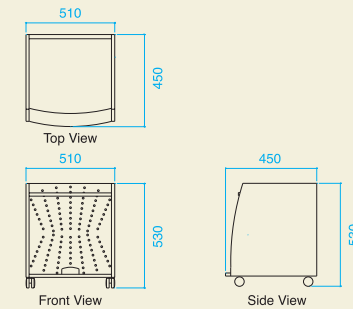
MPC 450 (473x457x608)
