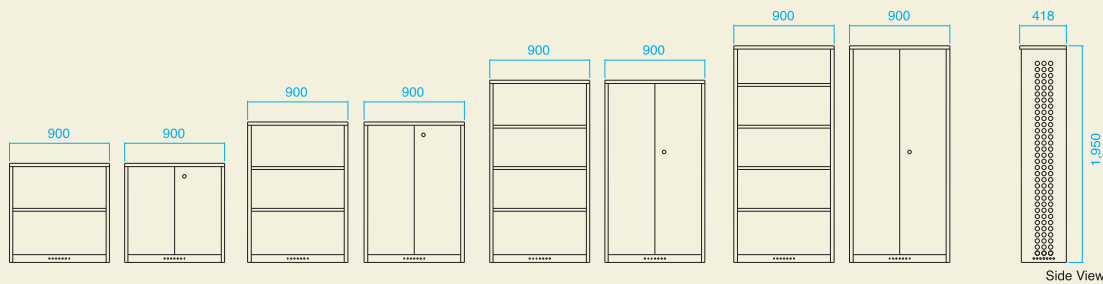
MPCD090 (900x417x900)
