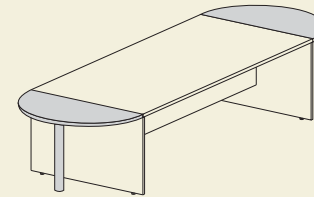
MKCN 012 (1200x600x740)
