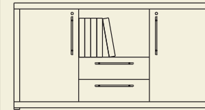
NODD 0917 (1700x900x400mm)
