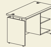
MKCD 120 (1200x600x725)
