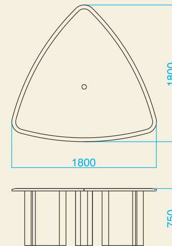
ITCO 180 (1800x1800x750mm)
