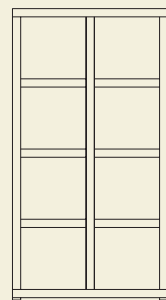
NOC 090 (900x1775x400mm)
