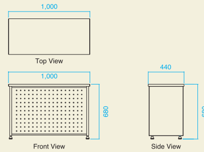
MPS 100 (1000x440x680)
